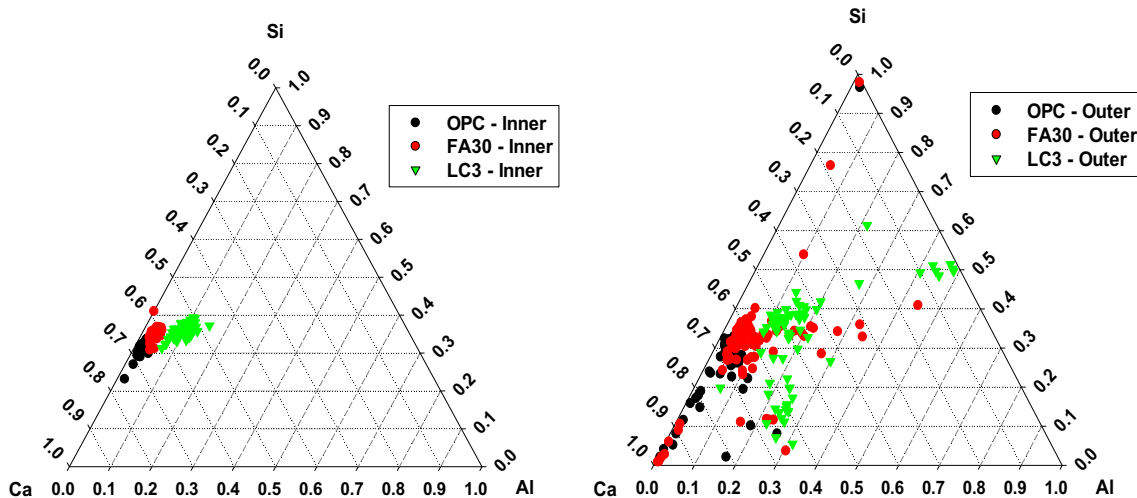
Fig. 14. Composition of inner and outer CSH in the OPC, FA30, and LC 3 cementitious systems at 150 days.
