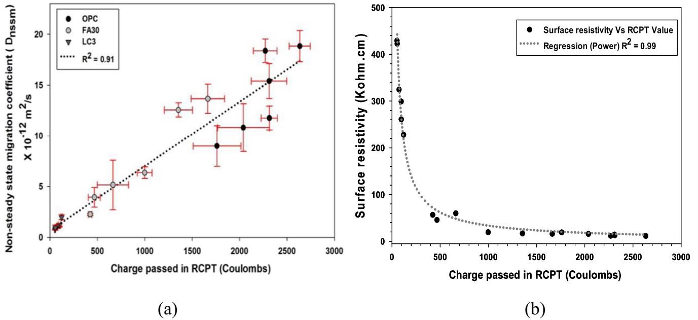
Fig. 11. a) Chloride penetration resistance of different binders evaluated by RCPT and ACMT, and b) correlation between surface resistivity and charge passed in RCPT.
