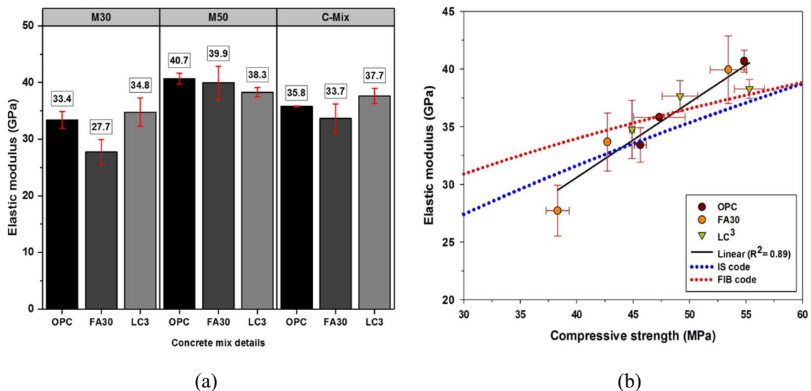
Fig. 3. (a) Elastic moduli of concretes made with OPC, FA30, and LC 3 and (b) correlation between elastic modulus and compressive strength.
