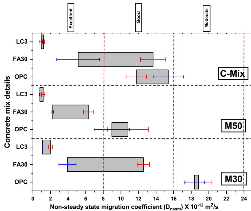
Fig. 10. Chloride migration coefficient of the different concretes at 28 days (red) and 90 days (blue). (For interpretation of the references to colour in this figure legend, the reader is referred to the web version of this article.)
